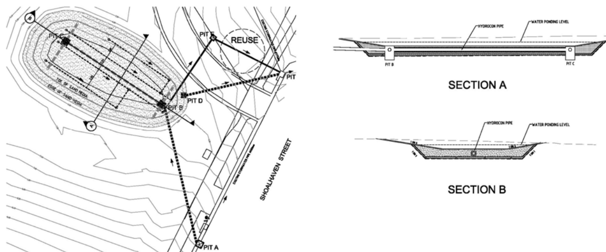
Figure 2: Sand filter design
